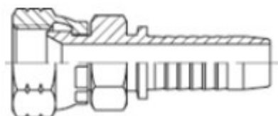
Hydraulic Toyota BSP threaded fittings Inner Y form cone – 60° Standard – JIS 8363 *- not stock
