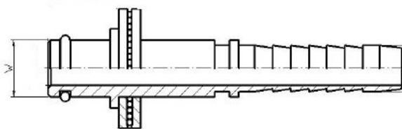
Pressure fittings-tube for high pressure washing with bearing *-not stock
