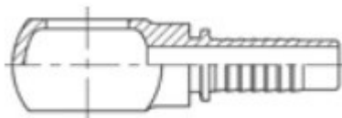
Pressures hydraulic fittings – banjo RNM with metric hole Standard – DIN7642 *-not stock
