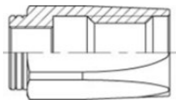
Assemble ferrules for hydraulic not skive hoses 1SN and 2SN
