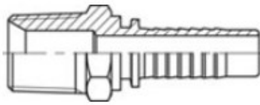
Hydraulic AGK-K BSPT male tapered fittings Sealing thread Standard – BS 5200 (ISO 228-1) *-not stock
