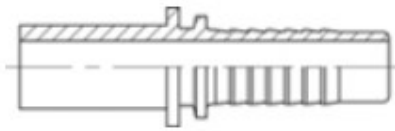
Pressure hydraulic fittings BEL/BES with tube Standard – DIN 2353 *-not stock
