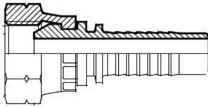
Pressure hydraulic fittings DKM Cone – 60° *-not stock
