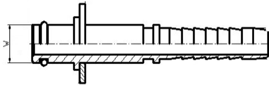
Pressure fittings-tube for high pressure washing *-not stock
